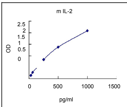
Figure 3: Representative standard curve for IL-2 ELISA. IL-2 was diluted in serial two-fold steps in Sample Diluent.
