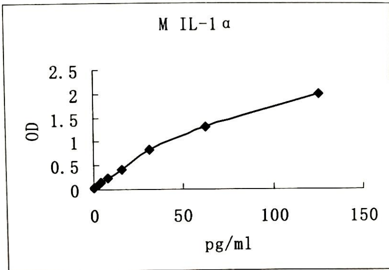
Figure 3: Representative standard curve for IL-1 \alpha ELISA. IL-1 \alpha was diluted in serial two-fold steps in Sample Diluent.
