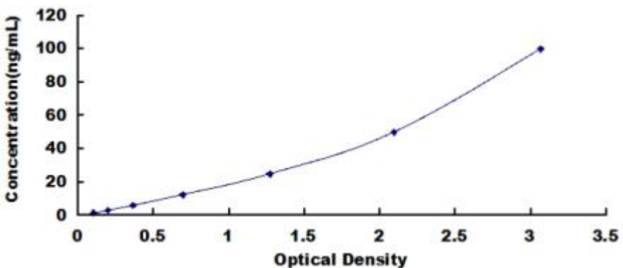
Typical Standard Curve for Rabbit SDC1 ELISA.
