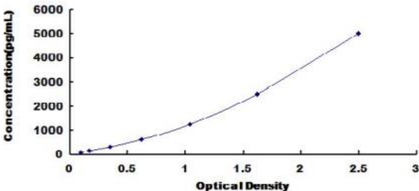
Typical Standard Curve for monkey APRIL ELISA.
