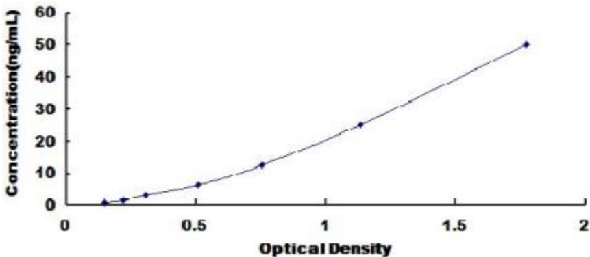
Typical Standard Curve for monkey HBB ELISA.
