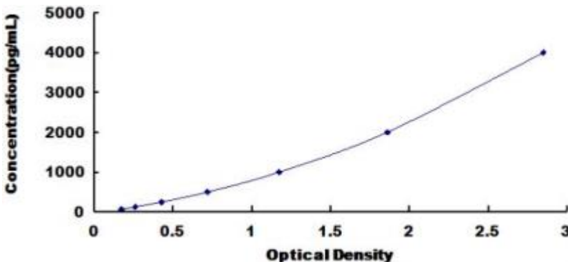
Typical Standard Curve for monkey QSOX1 ELISA.
