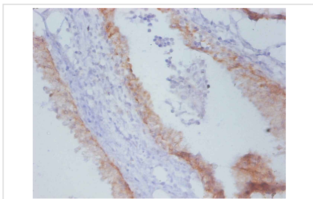
Immunohistochemical analysis of paraffin-embedded Rat prostate cancer using #42048 at dilution of 1:100.
