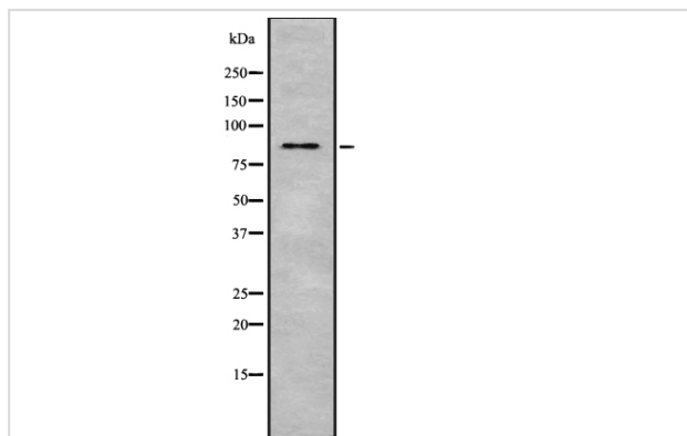
Western blot analysis ZBTB17 using HeLa whole cell lysates
