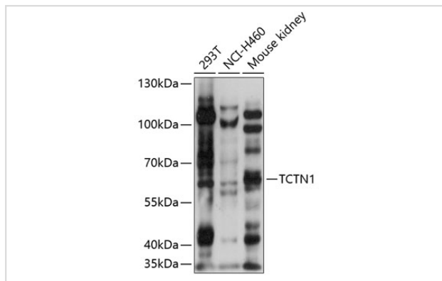
Western blot analysis of extracts of various cell lines, using TCTN1 antibody.
