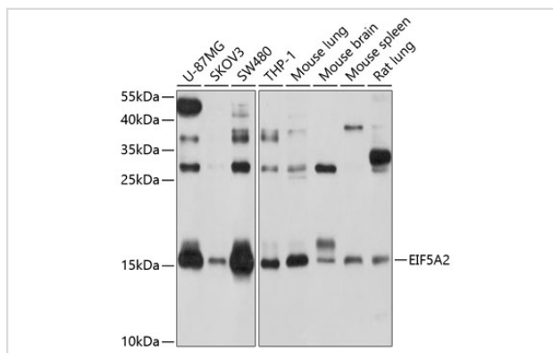
Western blot analysis of extracts of various cell lines, using EIF5A2 antibody.
