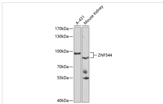
Western blot analysis of extracts of various cell lines, using ZNF544 antibody at 1:1000 dilution.
