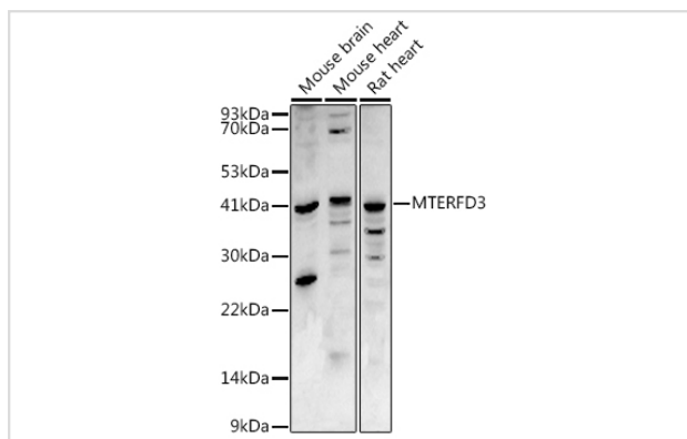
Western blot analysis of extracts of various cell lines, using MTERFD3 antibody.
