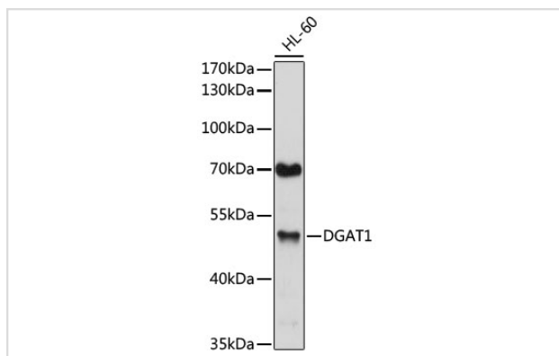
Western blot analysis of extracts of various cell lines, using DGAT1 at 1:1000 dilution.
