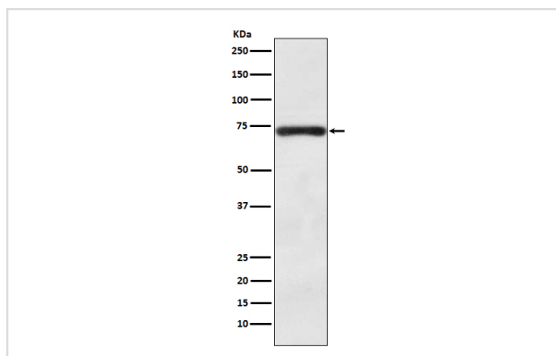
Western blot analysis of BACE1 expression in SH-SY5Y cell lysate.
