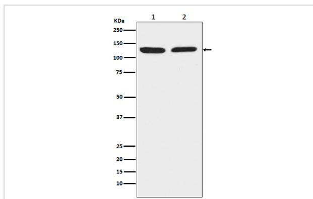
Western blot analysis of Chromogranin B expression in (1) HeLa cell lysate; (2) Raw 264.7 cell lysate.
