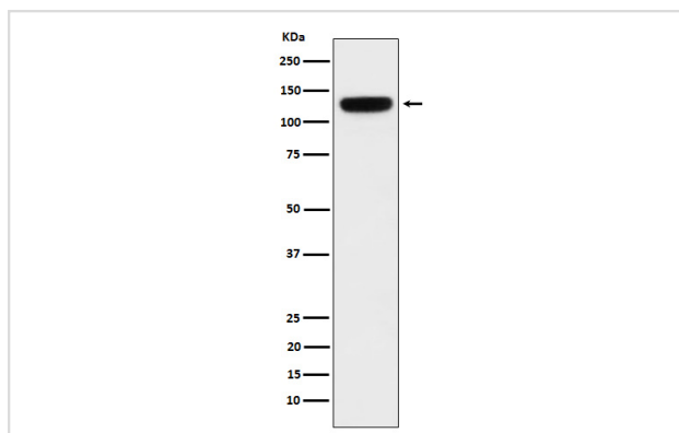
Western blot analysis of PER3 expression in K562 cell lysate.
