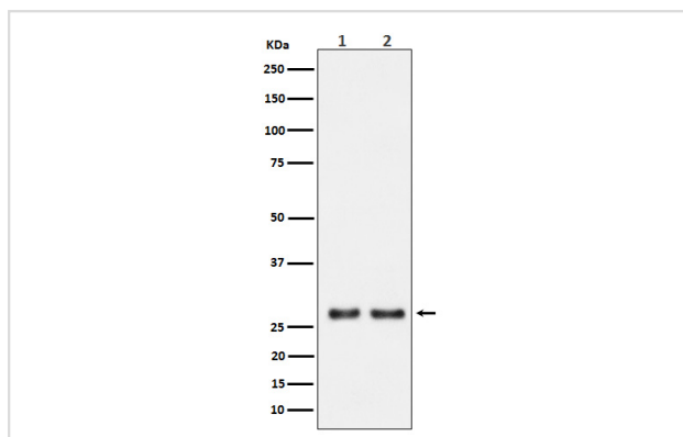
Western blot analysis of UPP1 expression in (1) HeLa cell lysate; (2) 293 cell lysate.
