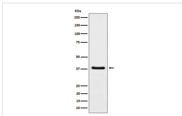
Western blot analysis of HDGF expression in A549 cell lysate.
