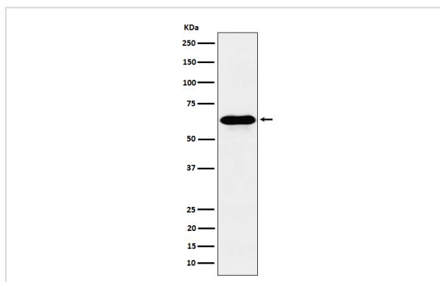
Western blot analysis of COASY expression in HeLa cell lysate.
