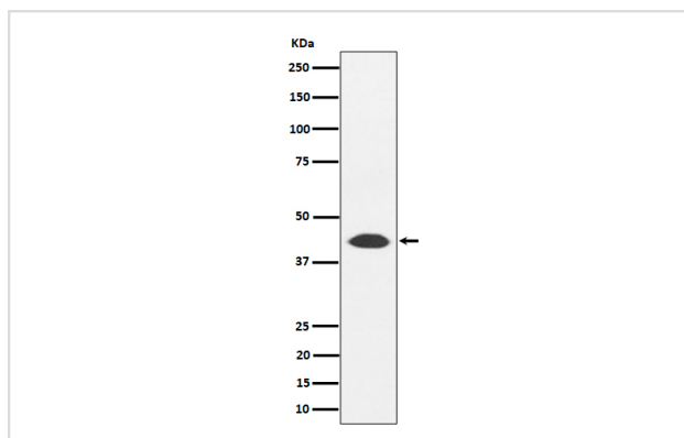
Western blot analysis of NUDT19 expression in 293T cell lysate.
