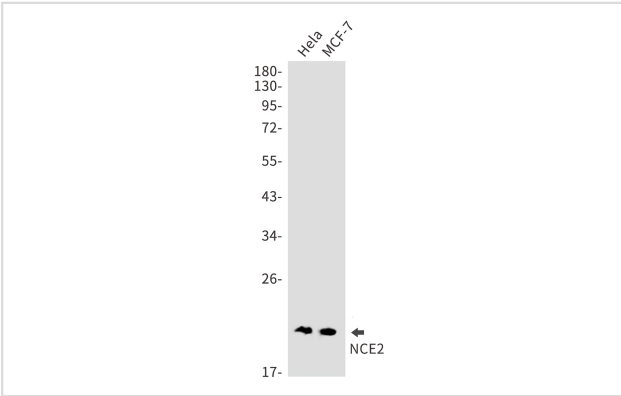
Western blot analysis of NCE2 in HeLa, MCF-7 lysates using NCE2 antibody.
