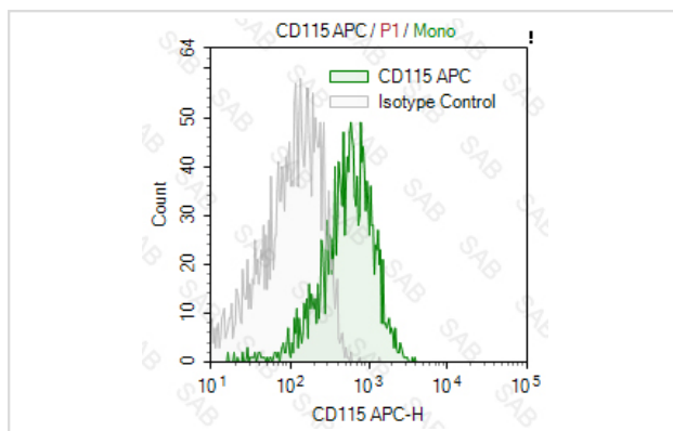
Human peripheral blood monocytes stained with APC anti-human 115 (colored histogram) or APC Rat IgG1 κ (gray histogram)
