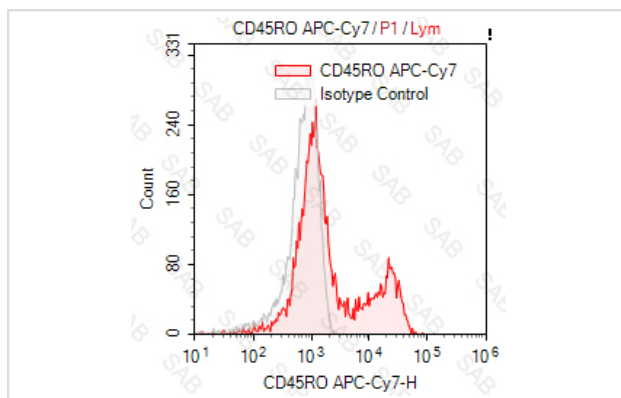
Human peripheral blood lymphocytes stained with APC-Cy7 anti-human CD45RO (colored histogram) or APC-Cy7 mouse IgG2a κ (gray histogram)
