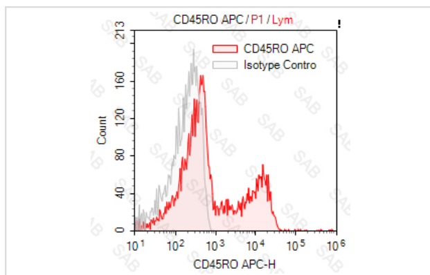
Human peripheral blood lymphocytes stained with APC anti-human CD45RO (colored histogram) or APC mouse IgG2a κ (gray histogram)
