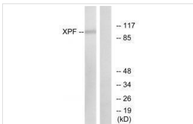
Western blot analysis of extracts from 293 cells, using XPF antibody #33545.
