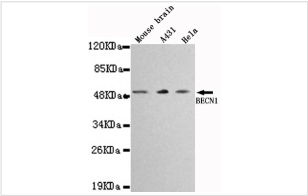
Western blot detection of BECN1 in Mouse brain,A431&Hela cell lysates using BECN1 antibody (1:1000 diluted). Predicted band size:52KDa. Observed band size:55KDa
