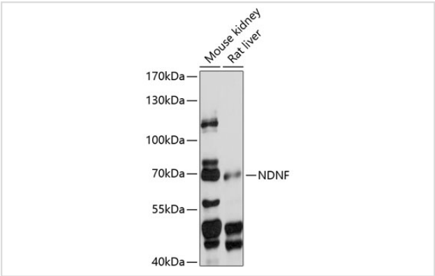
Western blot analysis of extracts of various cell lines, using NDNF antibody.
