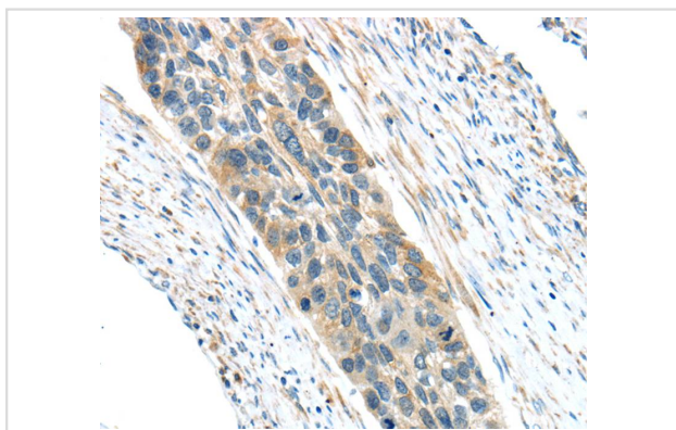
Immunohistochemical analysis of paraffin-embedded Human esophagus cancer tissue using #40403 at dilution 1/30.
