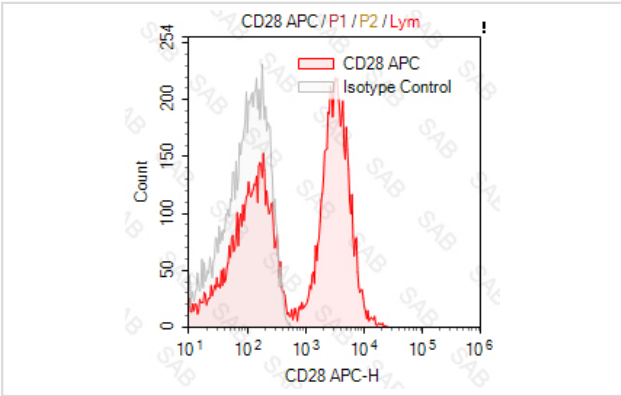
Human peripheral blood lymphocytes stained with APC anti-human CD28 (colored histogram) or APC mouse IgG1 κ (gray histogram)
