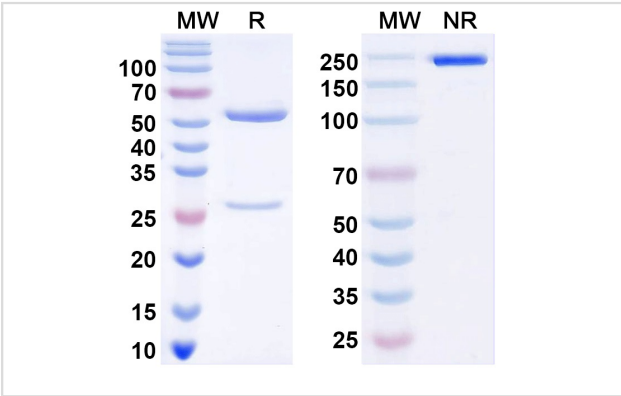
SDS-PAGE for Anti-Influenza A virus/Flu-A Monoclonal Antibody
