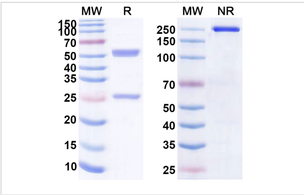
SDS-PAGE for Anti-HPV39 E7/Protein E7 Antibody
