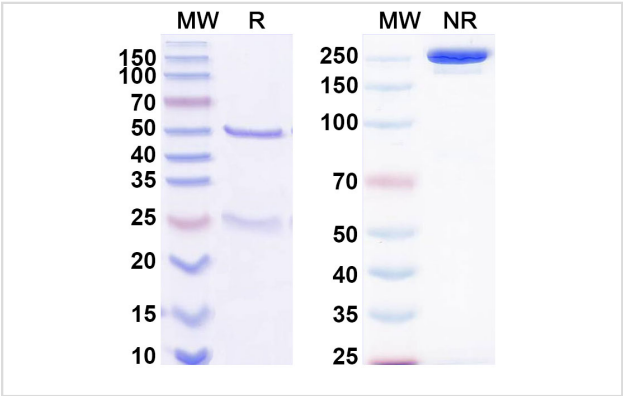
SDS-PAGE for Anti-HPV51 E7/Protein E7 Antibody
