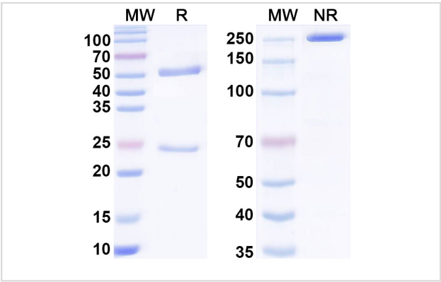
SDS-PAGE for Anti-G-quadruplex DNA Antibody
