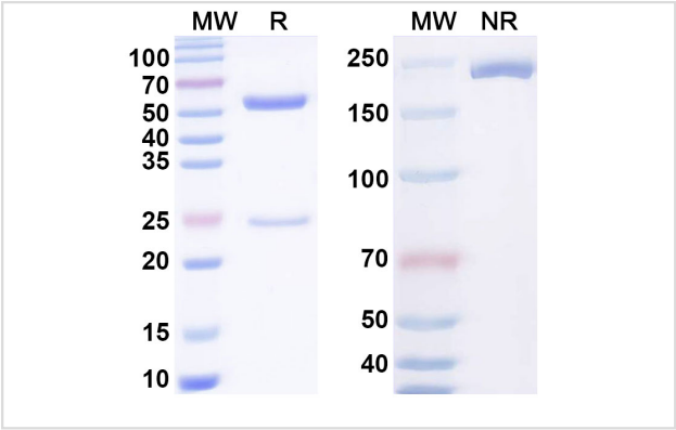
SDS-PAGE for Anti-Hairpin ssDNA Antibody .
