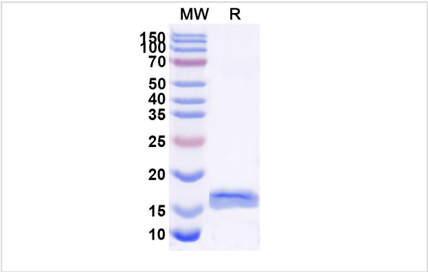
SDS-PAGE for Anti-DNA G-quadruplex Structures Nanobody
