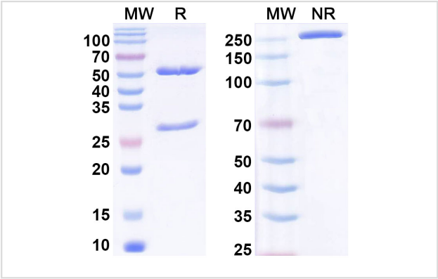
SDS-PAGE for Anti-RNA Antibody .
