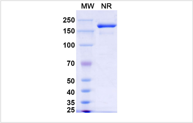
SDS-PAGE for Anti-dsRNA Recombinant Antibody
