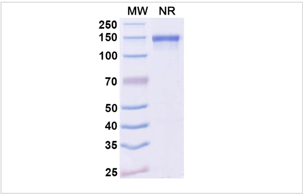
SDS-PAGE for Anti-Dupilumab Neutralizing Antibody
