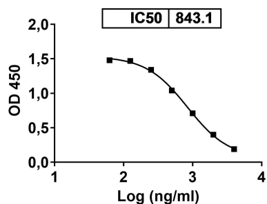
Anti-Pertuzumab Neutralizing Antibody (AD2137) Blocking with ERBB2
