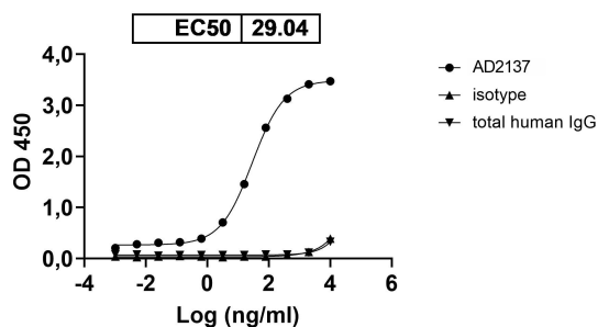
Anti-Pertuzumab Neutralizing Antibody (AD2137) binds with Pertuzumab
