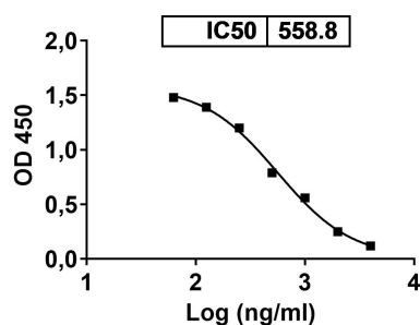
Anti-Pertuzumab Neutralizing Antibody (AD2009) Blocking with ERBB2
