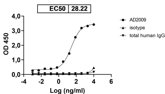
Anti-Pertuzumab Neutralizing Antibody (AD2009) binds with Pertuzumab
