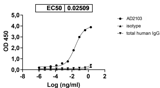
Anti-Pertuzumab Neutralizing Antibody (AD2103) binds with Pertuzumab
