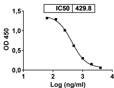
Anti-Pertuzumab Neutralizing Antibody (AD2103) Blocking with ERBB2
