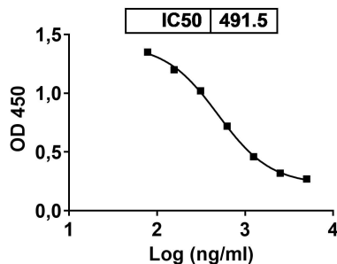
Anti-Tocilizumab Neutralizing Antibody (AD2234) Blocking with IL6R
