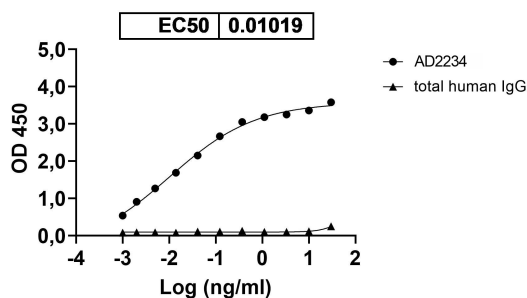
Anti-Tocilizumab Neutralizing Antibody (AD2234) binds with Tocilizumab
