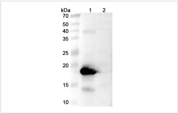
Lane 1: recombinant European white birch Bet v 1/Allergen Bet v I-A Lane 2: 1*loading buffer
