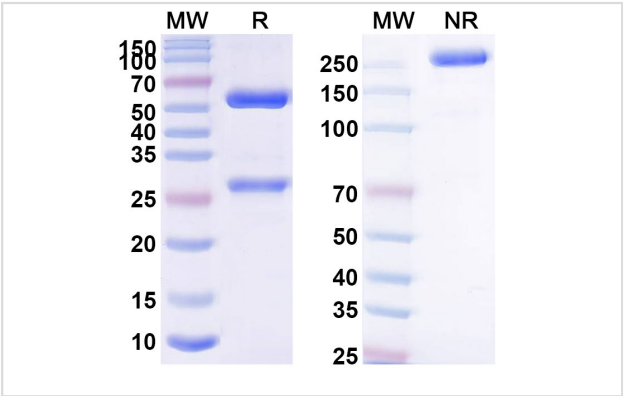
SDS-PAGE for Anti-BETVII/Allergen Bet v II Monoclonal Antibody
