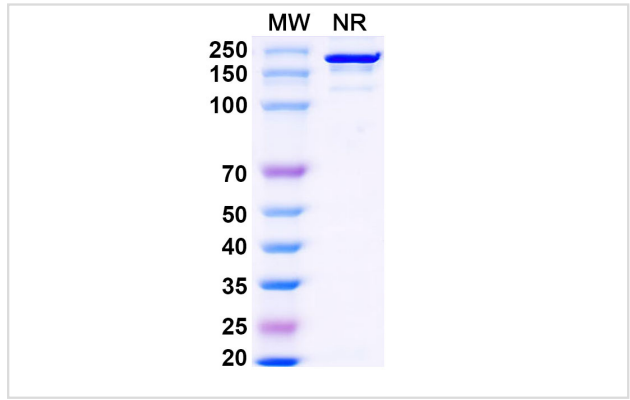
SDS-PAGE for Anti-Bovine Serum Albumin/BSA Antibody .
