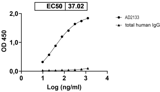
Anti-Ocrelizumab Non-Neutralizing Antibody (AD2133) binds with Ocrelizumab
