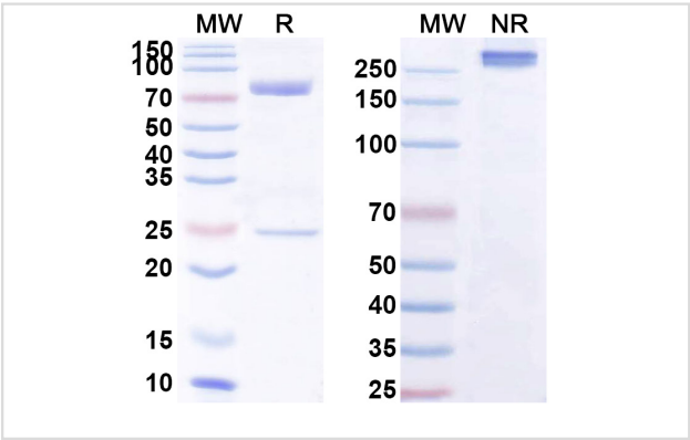
SDS-PAGE for Anti-Ganglioside GM1 hIgM Antibody
