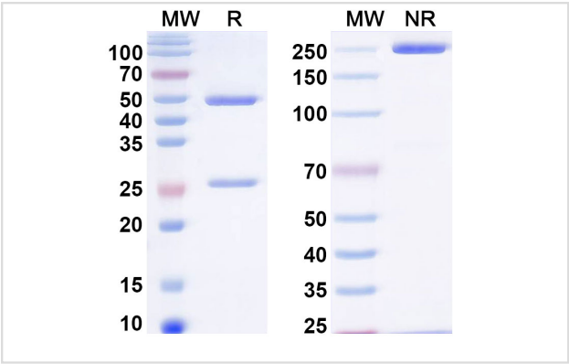
SDS-PAGE for Anti-Microcystin-LR/RR Antibody .
