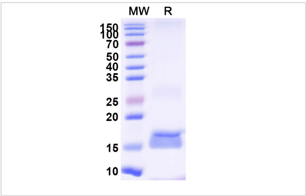
SDS-PAGE for Anti-Sahara scorpion AaH II/Neurotoxin II Nanobody
