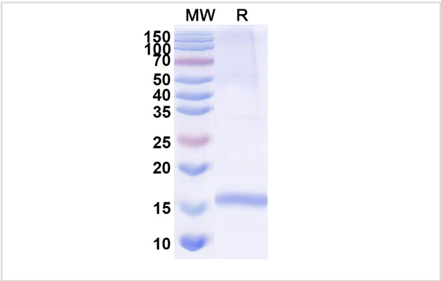
SDS-PAGE for Anti-Bacteriophage H19B stxB/SLT-1b/VT1 Nanobody
